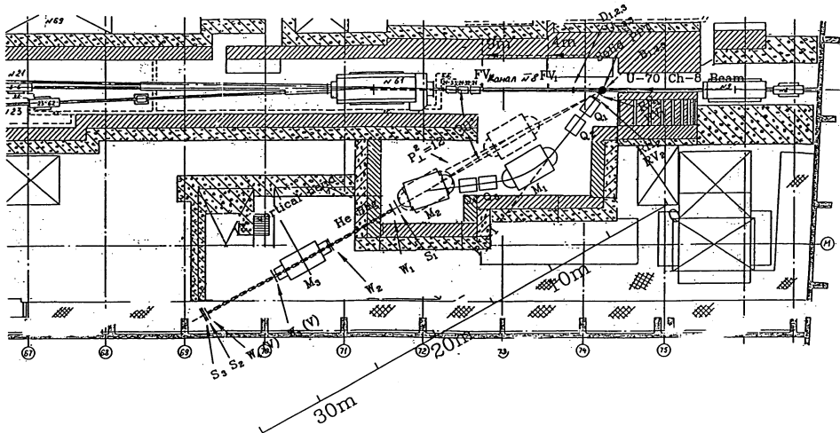
Spectrometer in U-70 Channel 8 Beam Line
