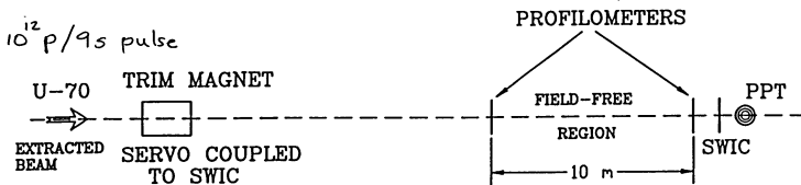
Figure 4. Sketch of beam-line system for stable centering of beam on target.
