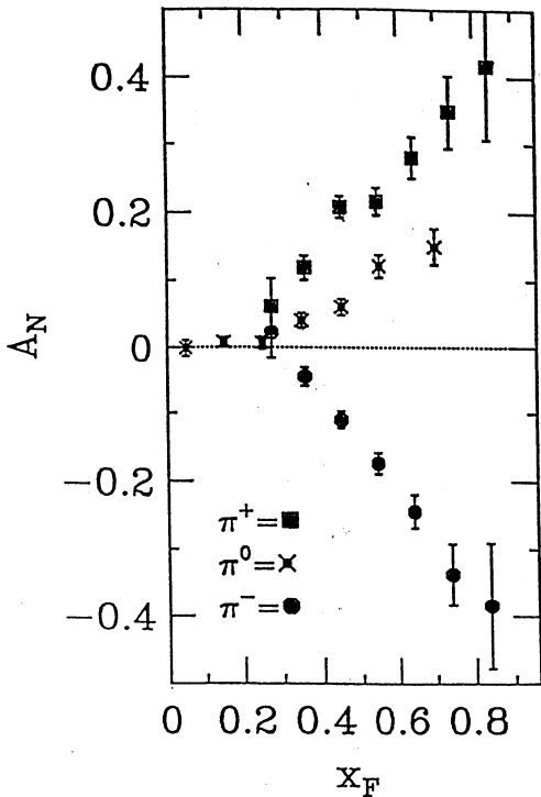
A_N for \pi^+ (squares) and \pi^- (circles) production in the p \uparrow p reaction versus x_F integrated over p_{\perp} . For comparison, \pi^0 data (crosses) are also plotted.
